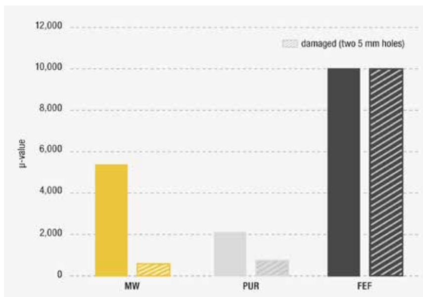
Figure 4: Resistance to water vapour transmission of the insulation materials after the test
